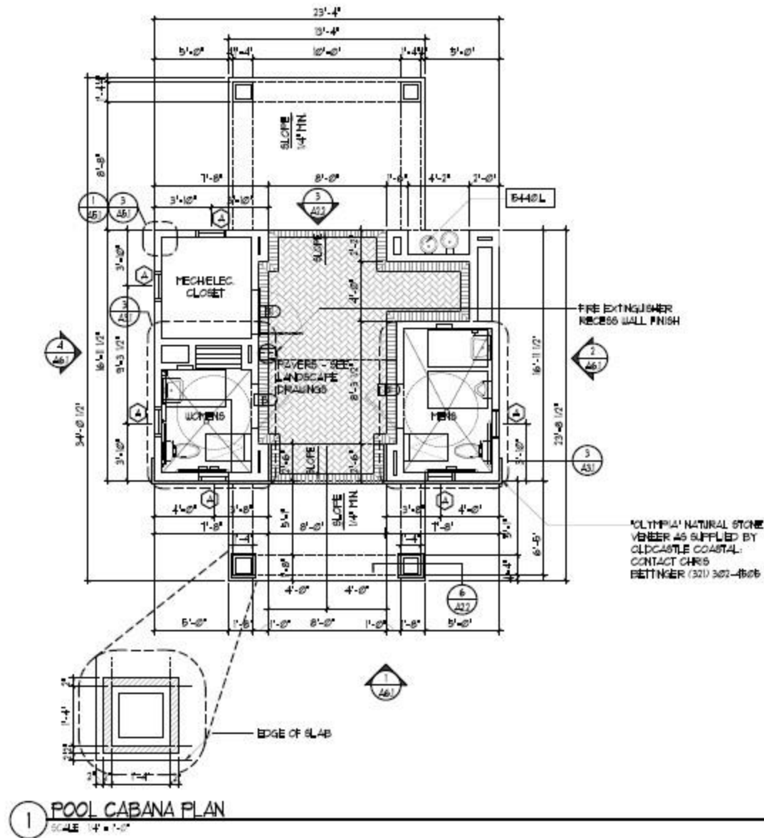
SHEET A2.1 POOL CABANA (FLOOR PLAN)
