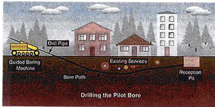
Figure 1: Drilling the pilot bore.
